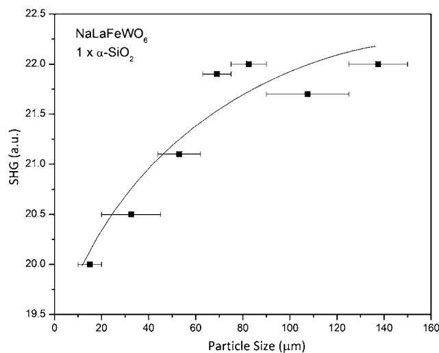
Figure 5. Powder second harmonic generation for NaLaFeWO 6 .
