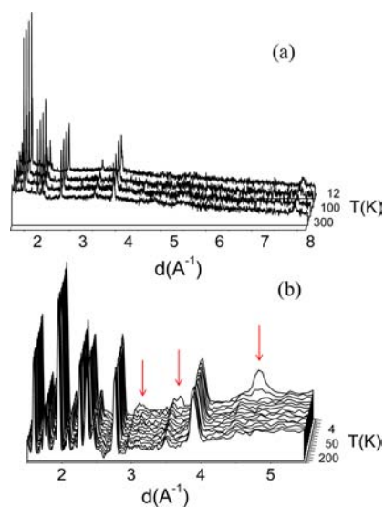
Figure 8. Thermal evolution of the PND patterns for (a) NaLaFeWO 6 and (b) NaNdFeWO 6 .
